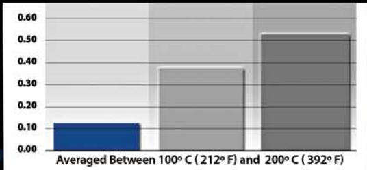
PAD WEAR 1000 Stop Normalized Akebono Pro-ACT OE Competitor Competitor B
