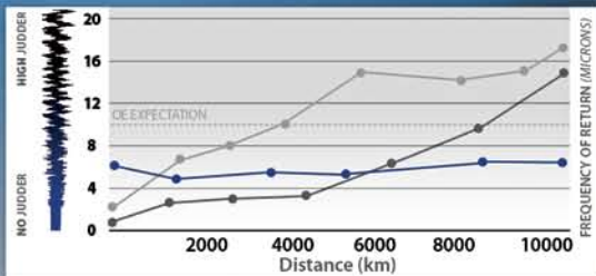
PEDAL PULSATION Tested at 0 to 10,000 km Akebono Pro-ACT OE Competitor Competitor A
