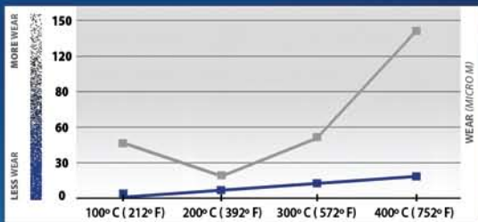
ROTOR WEAR 1000 Stop Normalized Akebono Pro-ACT OE Competitor
